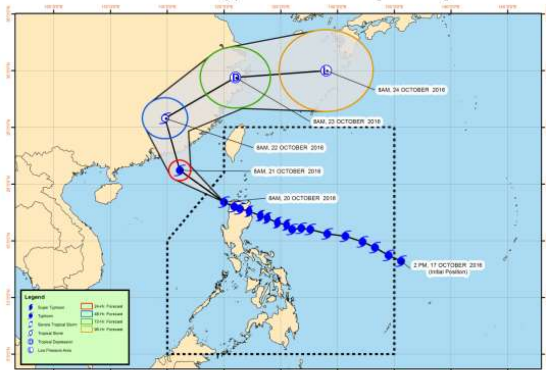
Track of Typhoon "LAWIN" [HAIMA]
